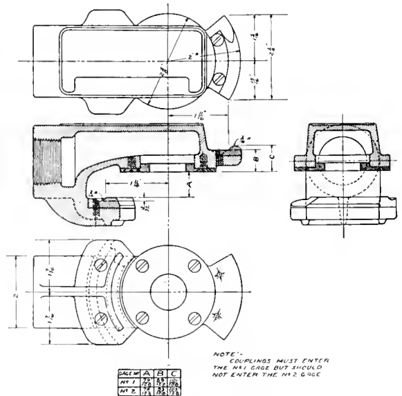
Fig. 1.—Gage for Air Brake Hose Couplings
